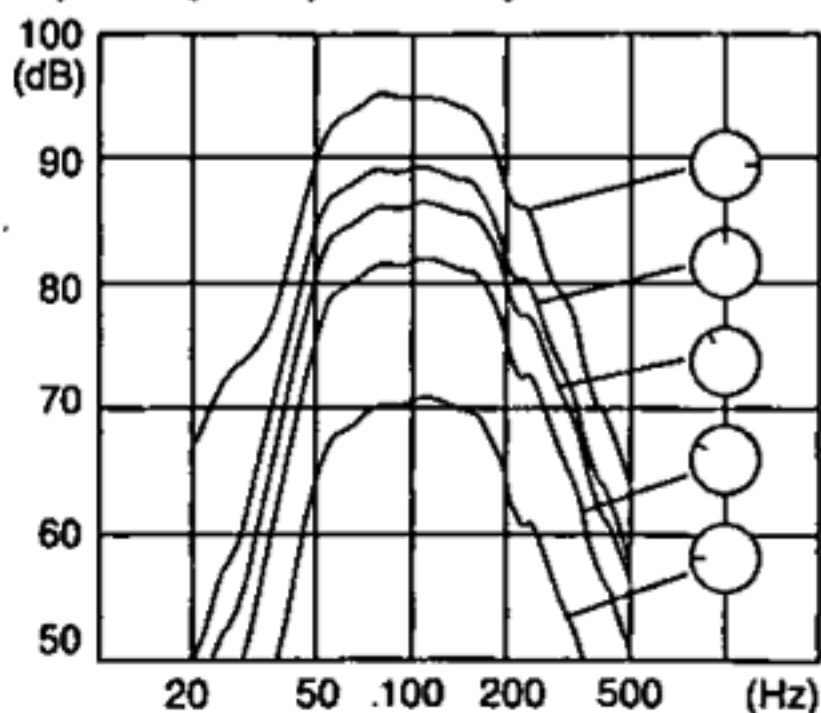
Frequency response by VOLUME setting
